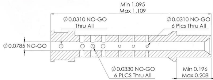
GX 160 DUMP TUBE
