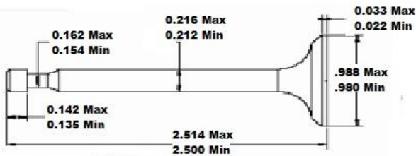
GX 160 Intake Valve
